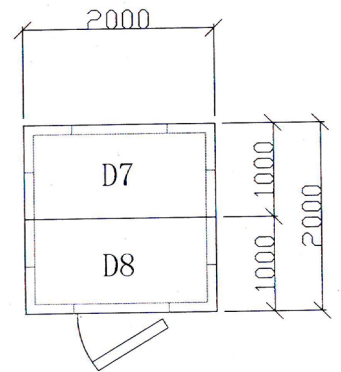
bottom panel
